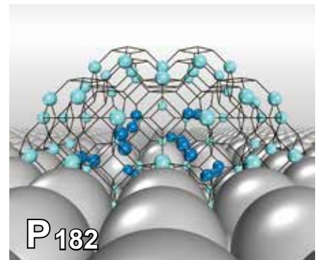
A new model depicts how hydrogen (cyan and blue atoms) nanobubbles are formed within metals, shedding lights on how metal failure is caused in certain hydrogen-enriched environments, such as tungsten armor in the core of a fusion reactor.
